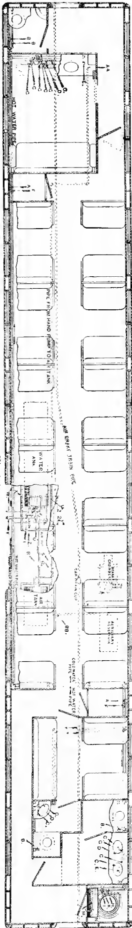
PULLMAN SYSTEM OF WATER SUPPLY FOR LAVATORIES AND CLOSETS. Hot and Cold Waters are Under Pressure of Compressed Air. Fig. 3541.
